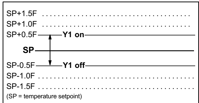
Figure 18. Cooling Mode
